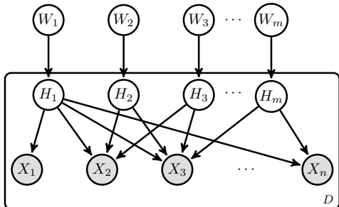
Figure 1. Graphical model representation of SPN \mathcal{S} . The box is a plate that represents replication over D training instances. m = O(|\mathcal{S}|) corresponds to the number of sum nodes and n is the number of observable variables in \mathcal{S} . Typically, m \gg n . W, H, X correspond to global latent variables, local latent variables and observable variables, respectively.
