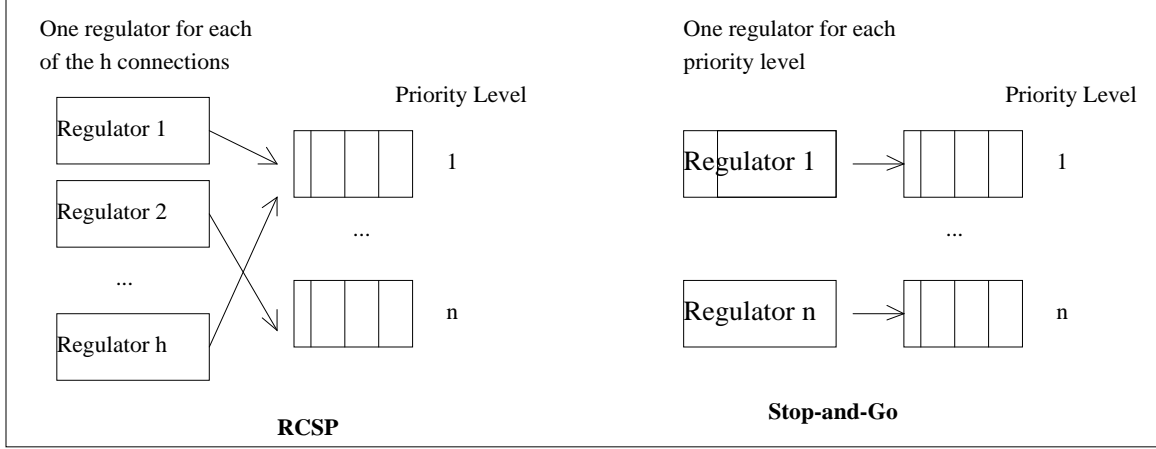
Figure 4: Stop-and-Go and RCSP
