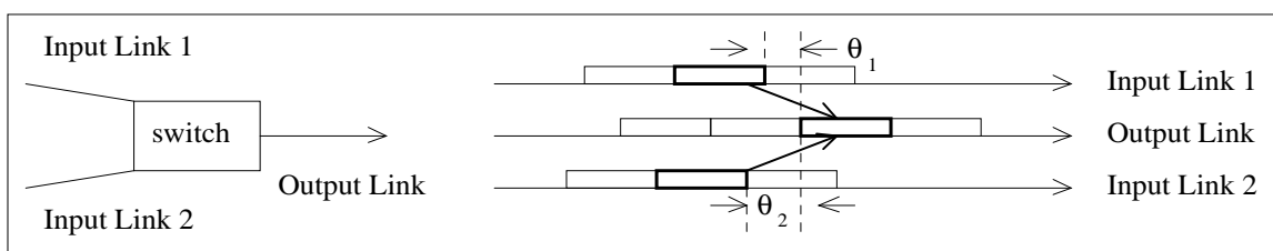
Figure 1: Synchronization between input and output links in Stop-and-Go
