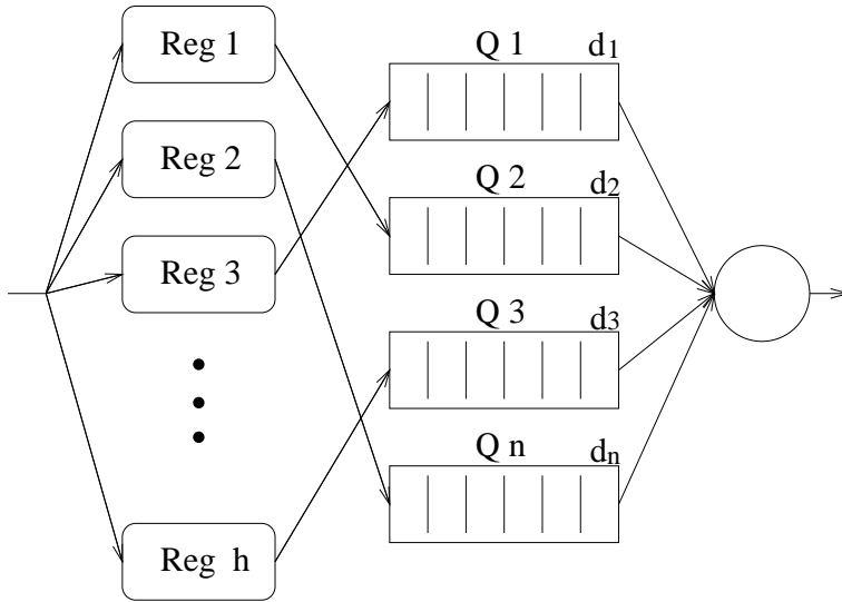
Figure 3: Rate-Controlled Static-Priority Queuing
