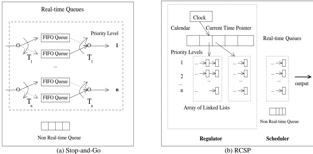
Figure 8: Implementation of RCSP and Stop-and-Go
