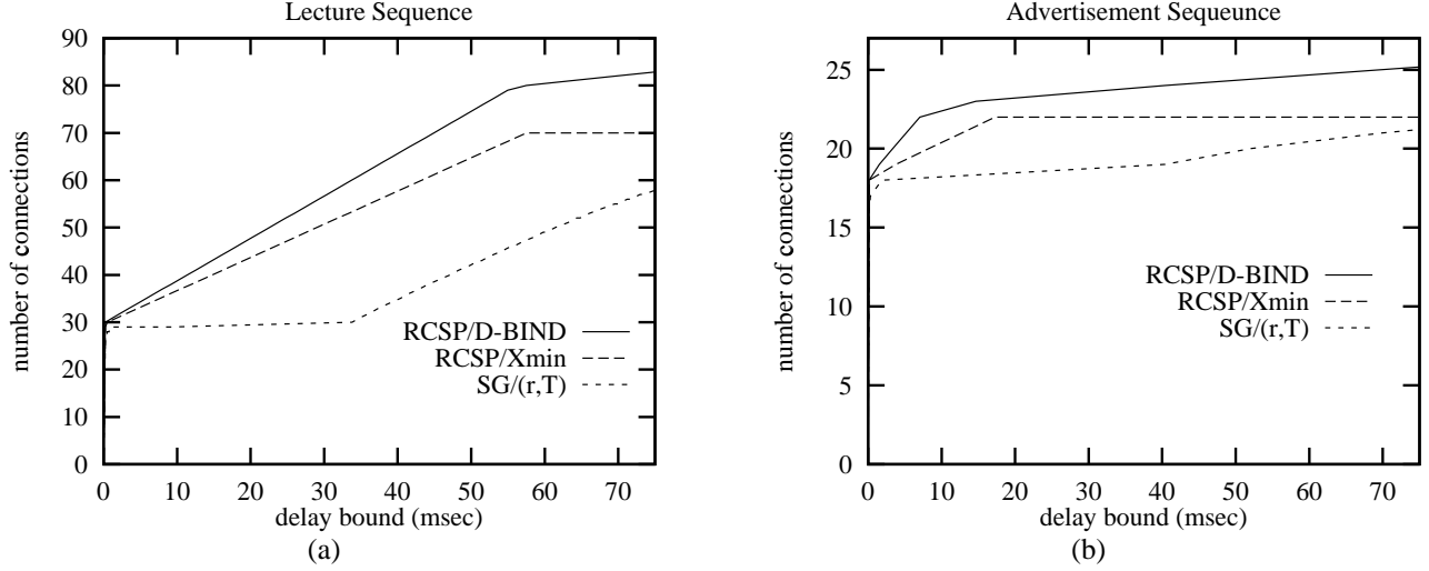
Figure 7: Connections Accepted vs. Delay Bound for SG and RCSP
