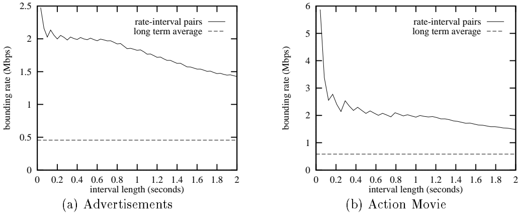
Figure 1: D-BIND Characterization of Advertisements and Action Movie
