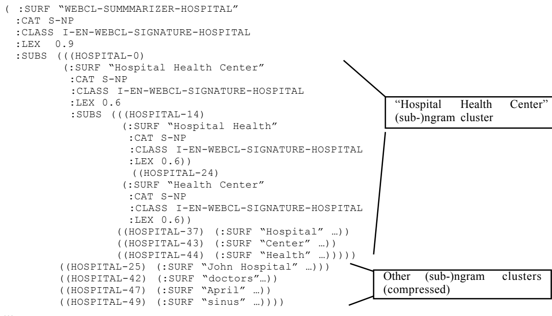
Figure 1. Portion of topic signature cluster tree for ngrams of "Hospital Health Center".
