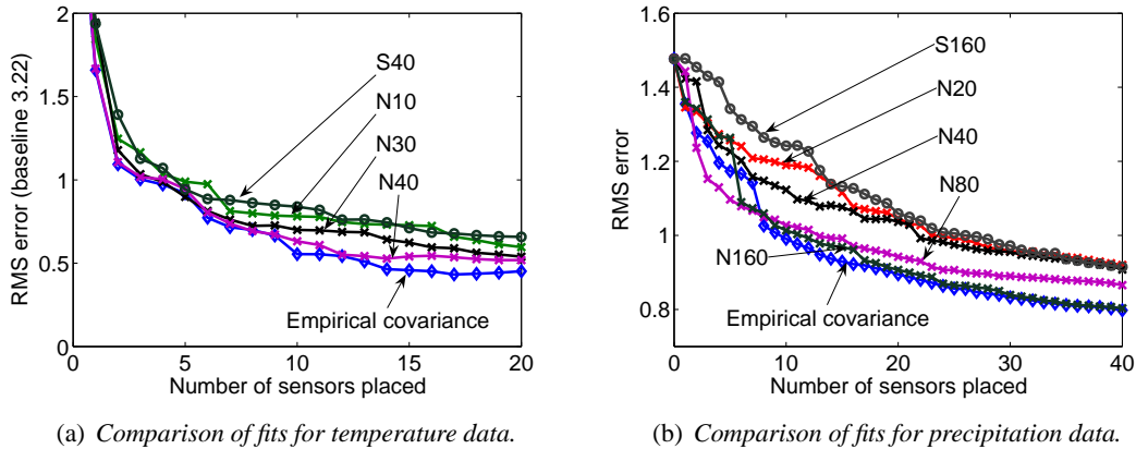
(a) Comparison of fits for temperature data. (b) Comparison of fits for precipitation data. Figure 9: RMS curves for placements of increasing size, optimized using stationary and nonstationary GPs. Prediction is done using estimated models. (a) Stationary GP estimated for the temperature data from 40 sensors (S40), nonstationary GPs estimated from 10, 30 and 40 sensors (N10, N30, N40). (b) Stationary GP estimated for the precipitation data from 160 sensors (S160), nonstationary GPs estimated from 20, 40, 80 and 160 sensors (N20, N40, N80, N160).
