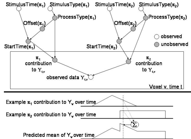
Figure 1. Top: A Hidden Process Model drawn as a graphical model. The observed data Y_v,t for voxel v at time t depends on contributions from some set of process instances (in this case \pi_1 and \pi_2 ). The contribution from a process instance depends on its start time and its process type. The process type references a general process description which specifies a response signature, duration, and timing distribution for its instances. The process type and the start time of a process instance depend on input stimuli. Bottom: Hidden Process Models assume that the contributions of process instances sum linearly to produce the mean of a normal distribution governing Y_v,t . In this example, the response signature of the process type for \pi_1 in voxel v is a triangle shape, and the response signature of the process type for \pi_2 in voxel v is a square. These response shapes are placed in time according to the start times for \pi_1 and \pi_2 and summed to obtain the predicted mean in voxel v .
