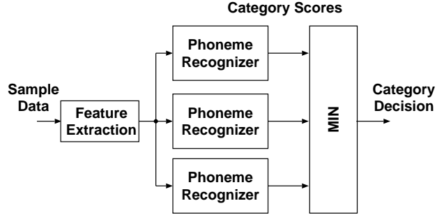
Fig. 1. Example age/ gender System based on Parallel Phoneme Recognizers (PPR) for 3 categories. The “MIN” decision selects the category pertaining to the phoneme recognizer yielding best (lowest) score.
