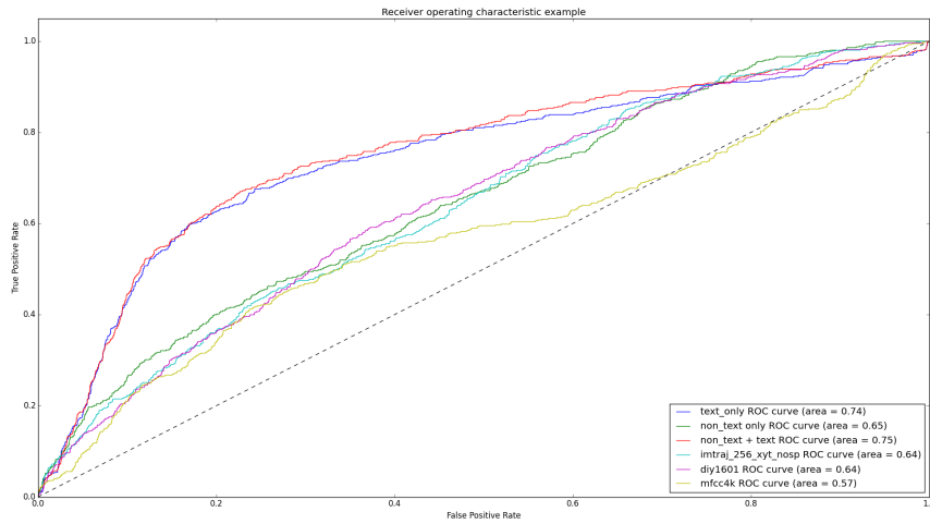
Figure 1: The ROC with Different Features on Development Dataset
