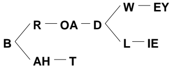
Figure 1: A simple pronunciation prefix tree (PPT) for a system using context-independent acoustic models.
