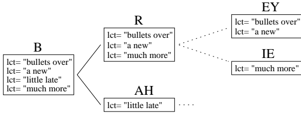
Figure 2: linguistic morphed instances within the PPT framework. (LCT= linguistic context)
