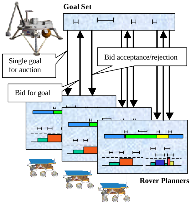
Figure 6. Contract Net Approach
