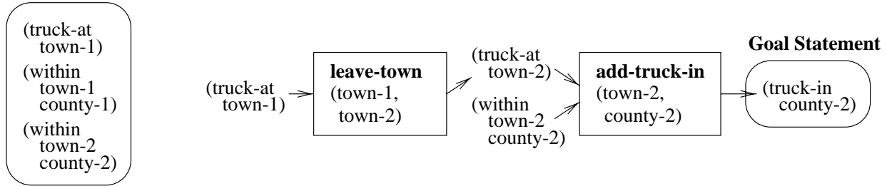
Figure 15: Use of an inference rule in backward chaining. PRODIGY links the add-truck-in rule to the goal literal and then adds leave-town to achieve the rule's precondition (truck-at town-2).
