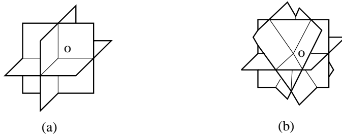
Figure 4: Orientation sets in three dimensions.
