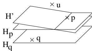
Figure 8: Proof of Lemma 3.
