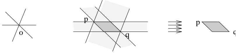
Figure 5: In two dimensions, the intersection of all the \mathcal{O} -oriented layers is the \mathcal{O} -block.
