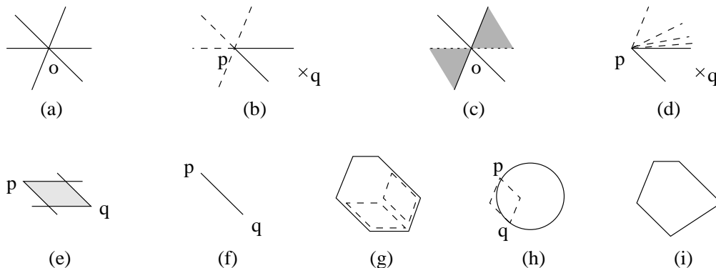
Figure 2: Planar strong convexity.
