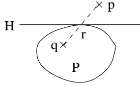
Figure 14: Proof of Theorem 18.
