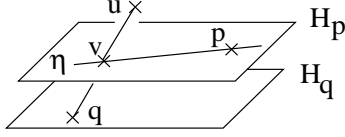
Figure 11: Proof of Theorem 12.
