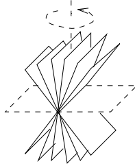
Figure 9: Construction of the orientation set \mathcal{O}_{sc} .
