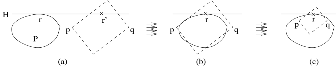
Figure 13: Proof of Theorem 17.
