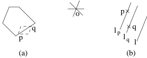
Figure 3: Proof of Lemma 2.
