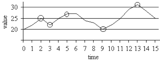
Figure 1 Example of a time series.
