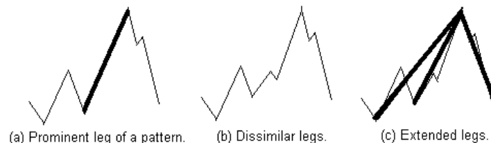
Figure 12 Example of extended legs. The pattern (a) matches the series (b), but the pattern's prominent leg has no equivalent in the series. If we identify the extended legs (c), the prominent leg matches one of them.
