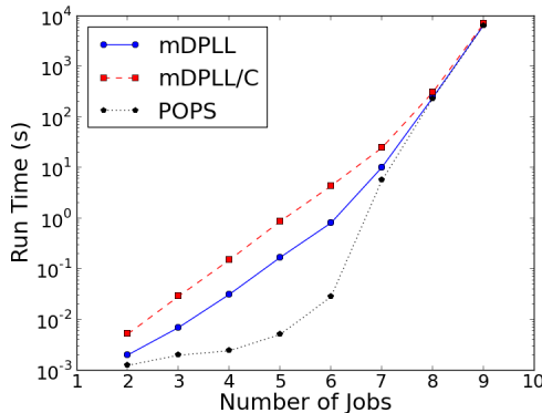
Figure 2: Log runtimes for #SAT job shop scheduling instances with 2 machines, 2 bits of uncertainty and 8 times steps.
