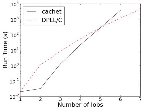
Figure 1: #SAT job shop scheduling problems with 2 machines, 2 bits of uncertainty and 4 times steps with varying numbers of jobs.
