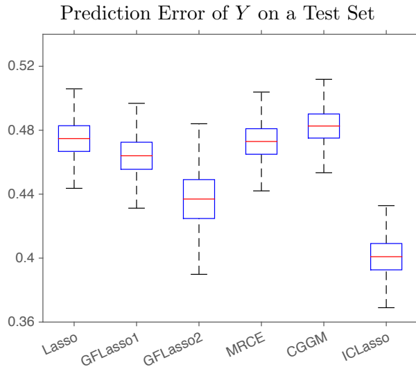
Figure 4: Test set prediction error on synthetic data with p = 60 , q = 120 , and a block-structured graph. Each box shows the mean (red), standard error interval (blue), and standard deviation (black) over 15 random datasets.
