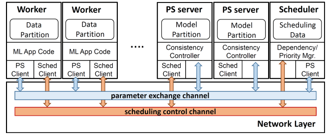
Figure 3: Petuum scheduler, workers, parameter servers.
