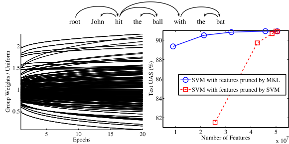
Figure 3: Top: a dependency parse tree (adapted from McDonald et al. 2005). Bottom left: group weights along the epochs of Alg. 3. Bottom right: results of standard SVMs trained on sets of feature templates of sizes \{107, 207, 307, 407, 507\} , either selected via a standard SVM or by MKL, via SPOM (the UAS— unlabeled attachment score —is the fraction of non-punctuation words whose head was correctly assigned.)
