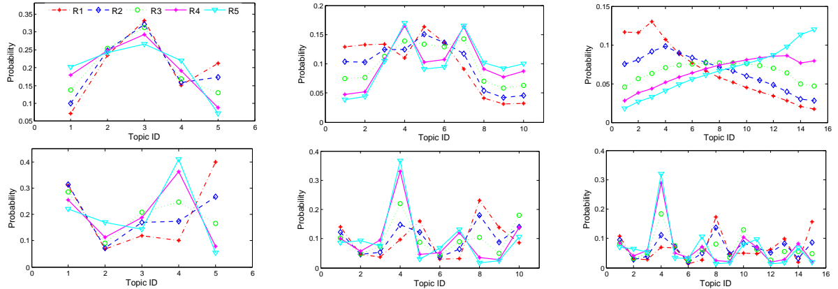
Figure 4. The average distribution over topics for documents of the same rating score. The top row is for max-margin sCTRF and the bottom row is for MedLDA. For each model, we use 5 (Left), 10 (Middle), and 15 (Right) topics.
