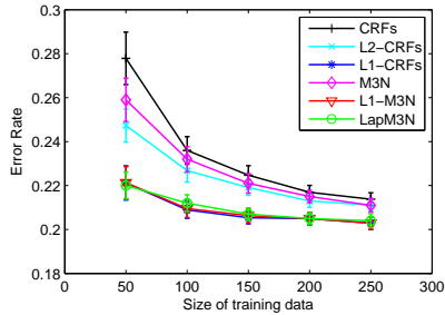
Figure 2: Error rates of different models.
