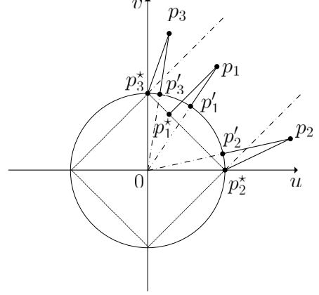
Figure 1: Projection of a point to the \ell_2 -ball (solid); and \ell_1 -ball (dashed) in the two-dimensional space.
