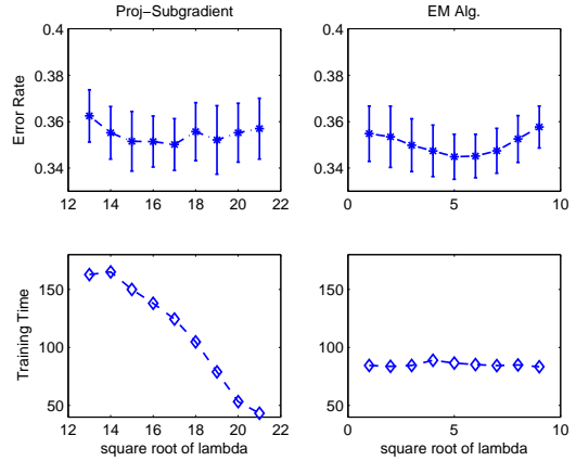
Figure 6: The error rates and training time (CPU-seconds) of different algorithms on the OCR100 data set against the regularization constants.
