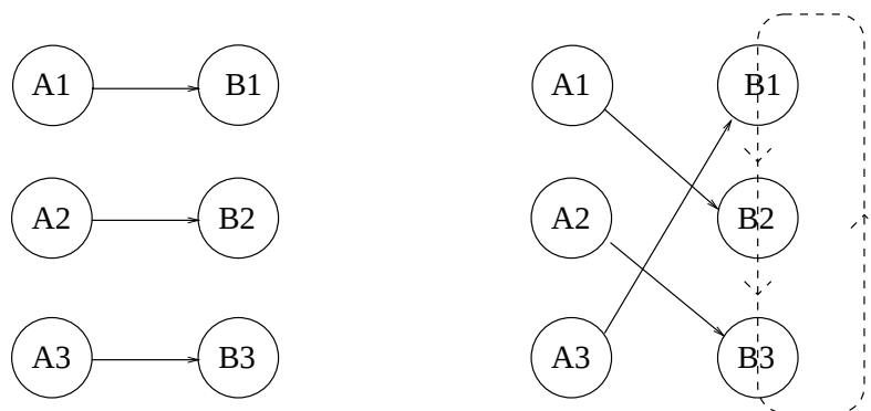
Fig. 11. Exploiting symmetry.
