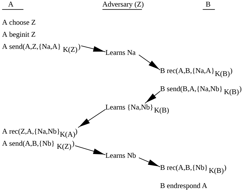
Fig. 2. Needham-Schroeder attack.
