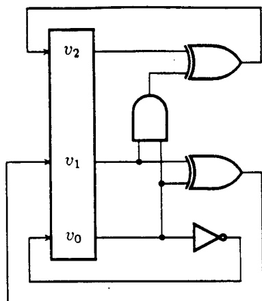
Figure 1. Synchronous modulo 8 counter.
