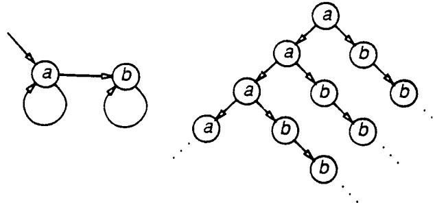
Figure 3. State transition graph and corresponding computation tree.
