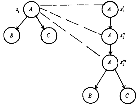
Figure 3-1: An Illustration of Corresponding Structures
