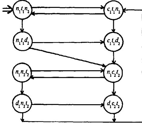
Figure 5-1: Two Process Mutual Exclusion Example
