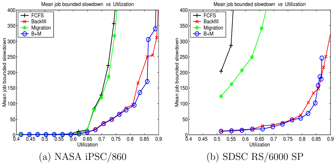
Figure 5-2: Mean job bounded slowdown vs utilization for (a) NASA and (b) SDSC logs.
