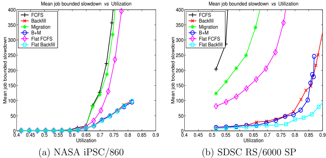
Figure 5-3: Mean job bounded slowdown vs utilization for the NASA and SDSC logs, comparing toroidal and flat machines.
