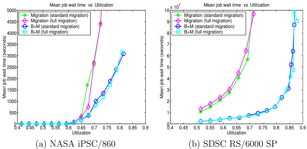
(a) NASA iPSC/860 (b) SDSC RS/6000 SP Figure 5-5: Mean job wait time vs utilization for the NASA and SDSC logs, comparing the standard migration policy to a full migration policy that always attempts to migrate.
