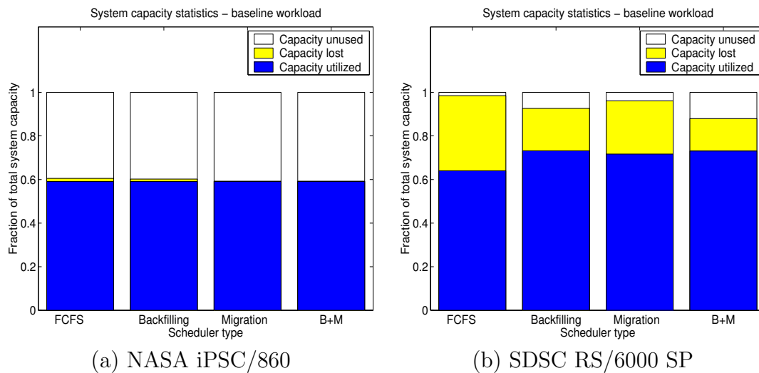
Figure 5-6: Capacity utilized, lost, and unused as a fraction of the total system capacity.
