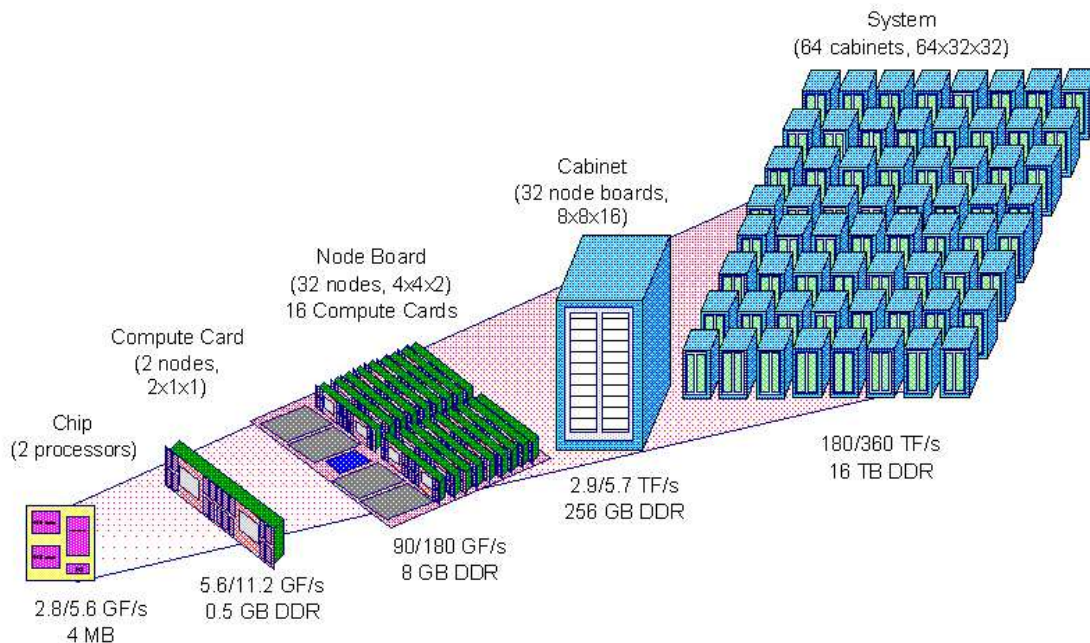
Figure 1-1: BlueGene/L architecture, with expected speed when utilizing 1 or 2 processors on each chip for computation
