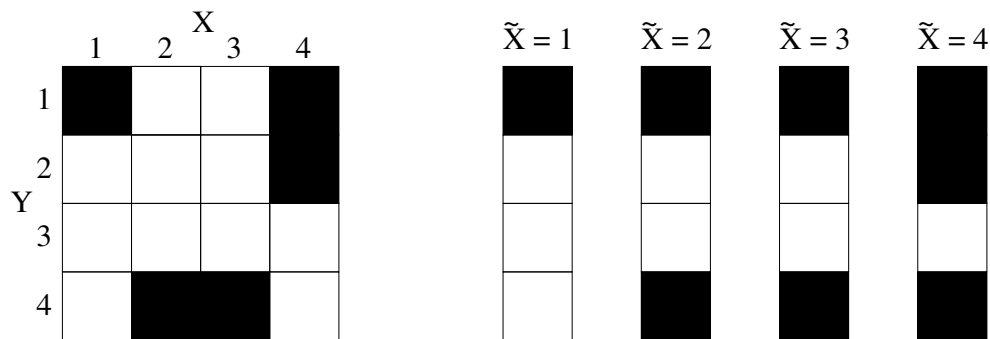
Figure 3-1: 2-dimensional POP Algorithm applied to Base Location (1,2): Adjacent 1-dimensional columns are projected onto each other as \tilde{X} is incremented.
