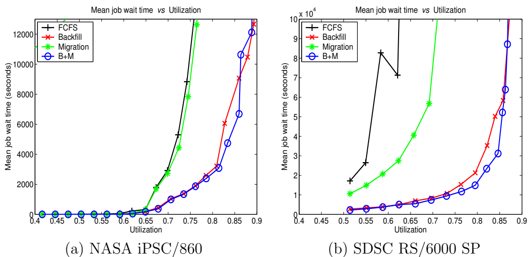
Figure 5-1: Mean job wait time vs utilization for (a) NASA and (b) SDSC logs.
