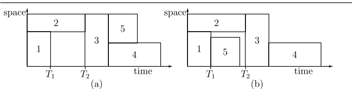
Figure 2-1: FCFS policy without (a) and with (b) backfilling. Job numbers correspond to their position in the priority queue.
