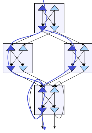
Figure 3.4: A GMCNF based representation of an register allocation with a sample allocation shown with the thicker line. Each block can be thought of as a crossbar where the cost of each edge is the shortest path between a given merge and split node.
