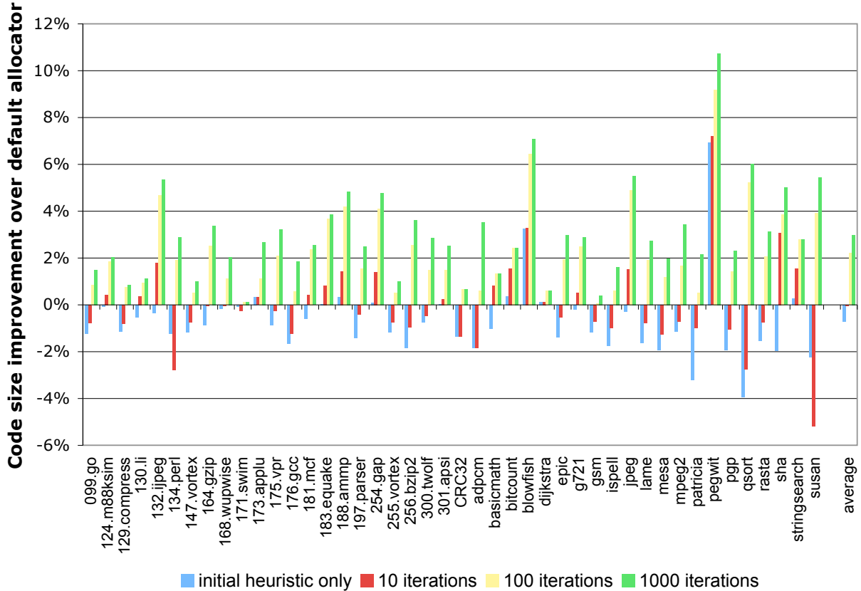
Figure 3.9: Code size improvement with our easy-update trace-based simultaneous allocator compared to the default allocator of gcc . All benchmarks were compiled using the -Os optimization flag. Our allocator outperforms the default allocator on all benchmarks after 100 iterations. The benchmark pegwit had the largest improvement with a size improvement of 10.78% after 1000 iterations.
