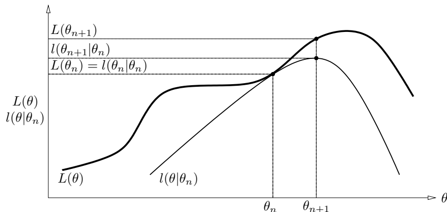
Figure 1: Graphical interpretation of a single iteration of the EM algorithm: The function L(\theta|\theta_n) is upper-bounded by the likelihood function L(\theta) . The functions are equal at \theta = \theta_n . The EM algorithm chooses \theta_{n+1} as the value of \theta for which l(\theta|\theta_n) is a maximum. Since L(\theta) \geq l(\theta|\theta_n) increasing l(\theta|\theta_n) ensures that the value of the likelihood function L(\theta) is increased at each step.
