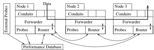
Figure 3: The RON system architecture. Data enters the RON from RON clients via a conduit at an entry node . At each node, the RON forwarder consults with its router to determine the best path for the packet, and sends it to the next node. Path selection is done at the entry node, which also tags the packet, simplifying the forwarding path at other nodes. When the packet reaches the RON exit node , the forwarder there hands it to the appropriate output conduit, which passes the data to the client. To choose paths, RON nodes monitor the quality of their virtual links using active probing and passive observation. RON nodes use a link-state routing protocol to disseminate the topology and virtual-link quality of the overlay network.
