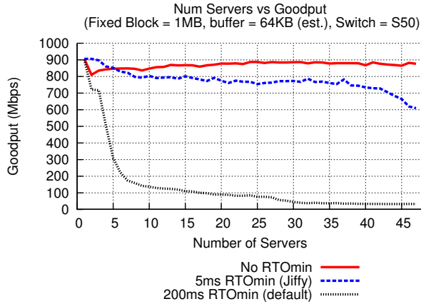
Figure 10: For a 48-node cluster, providing TCP retransmissions in microseconds eliminates incast collapse for up to 47 servers.
