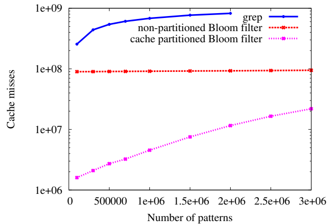
Fig. 10. Cache misses (measured with the Linux perf performance counters) when scanning the random ASCII corpus. Note the logarithmic scale on the Y axis.
