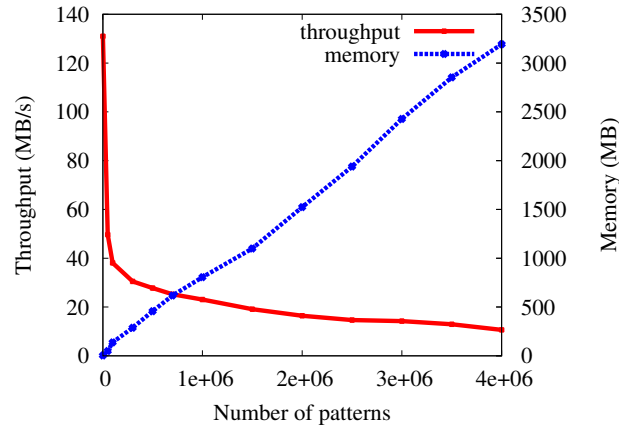
Fig. 1. The grep processing rate and memory consumption for various numbers of patterns. The average length of the patterns is 29 characters.
