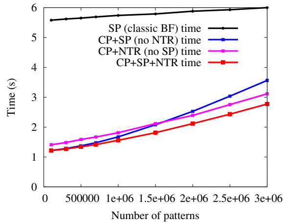
Fig. 8. The graph shows the benefit of each optimization: CP (cache-partitioning), SP (super pages), and NTR (non-temporal reads). The filters were run on 114 MB of random ASCII text, for different numbers of 19-character patterns. The cache-partitioned filters use five hash functions (two of which are for the cache-resident part) while the non-partitioned filter uses four. They are of similar size: 32 MB for the non-partitioned Bloom filter, and 2 + 32 MB for the cache-partitioned ones.
