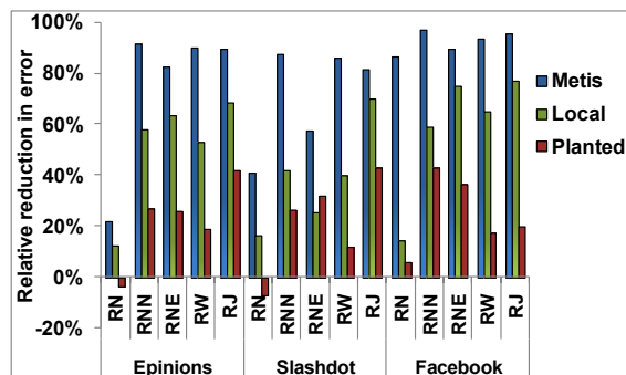
Figure 5. Reduction of error in the preservation of the clustering hierarchy, for UNWEIGHTED relative to INDUCED.
