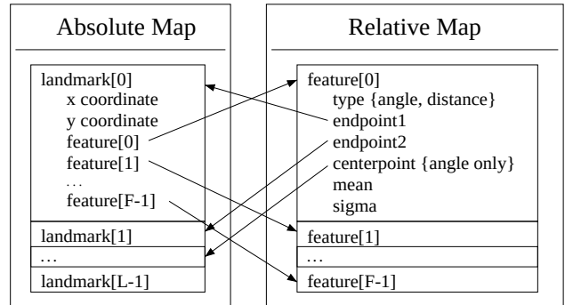
Figure 4: Relationship between absolute map and relative map data structures
