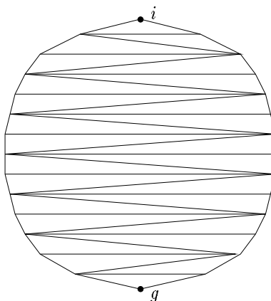
Figure 11: Example of a triangulation in which the shortest path is up to \frac{\pi}{2} times as long as the true shortest route.
