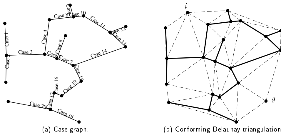
Figure 9: (a) Case graph (reproduced from Figure 2b). (b) Conforming Delaunay triangulation of case graph, for a particular initial vertex i and goal vertex g . Solid lines represent case edges, dashed lines represent other triangulation edges.
