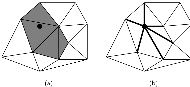
Figure 14: Inserting a new vertex into a Delaunay triangulation. (a) The shaded triangles are deleted because the new vertex is inside their circumcircles. (b) The new vertex is connected to its neighbors.
