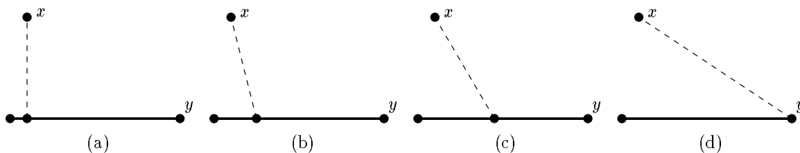
Figure 4: Examples of optimum routes between x and y for several \beta values. Solid lines are case segments, dotted lines are a portion of the optimum route. (a) \beta = 0 . (b) \beta = 0.25 . (c) \beta = 0.5 . (d) \beta \geq 0.83 .
