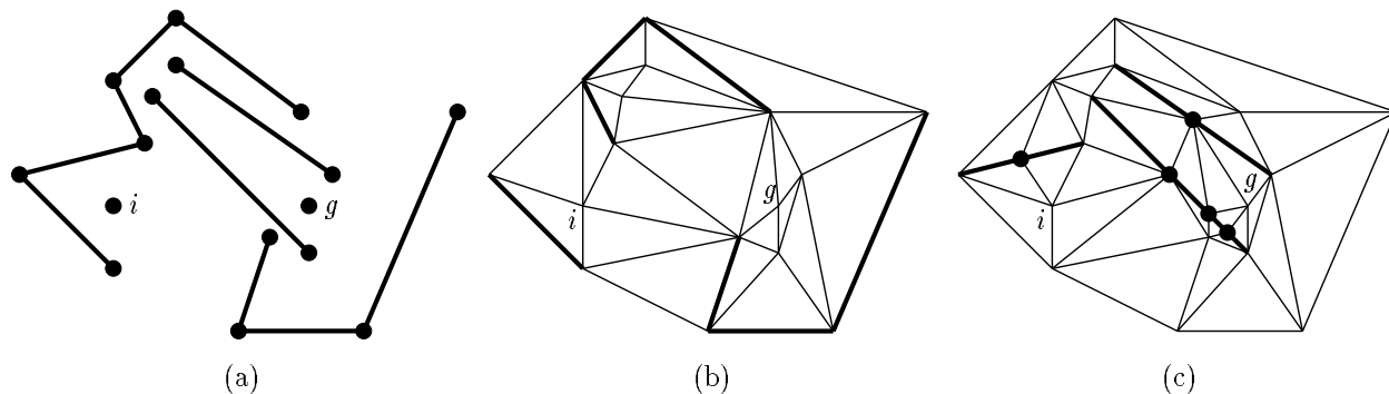
Figure 8: (a) Case graph. (b) Delaunay triangulation of the vertices of the case graph. Some case segments are represented by edges of the triangulation, but some are not. (c) A conforming Delaunay triangulation of the case graph. Additional vertices have been inserted to ensure that all case segments are represented.
