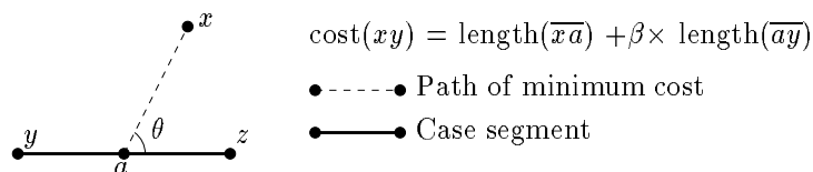
Figure 3: Finding the route of minimum cost.
