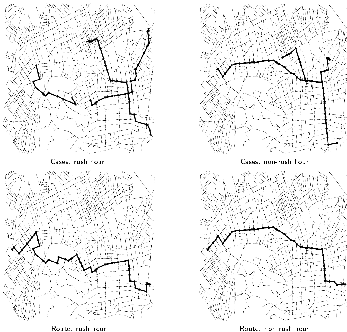
Figure 17: The relevant cases and the final route generated by PRODIGY/ANALOGY under different conditions.
