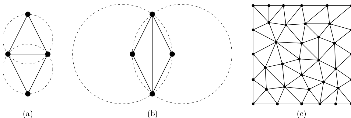
Figure 7: (a) A Delaunay triangulation of four vertices. The circumcircles of both triangles are illustrated. (b) Another triangulation (not Delaunay) of the same four vertices. (c) Example of a larger Delaunay triangulation. The Delaunay triangulation of a point set tends to connect vertices that are closer together.
