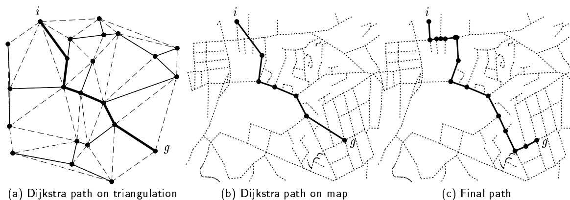
Figure 12: (a) The path found by Dijkstra’s algorithm in the Delaunay triangulation of Figure 9b; solid lines represent case edges, dashed lines represent triangulation edges, thick lines represent the path. (b) Dijkstra’s path superimposed on the real map. (c) Dijkstra’s path modified by PRODIGY/ANALOGY to conform to real world constraints.
