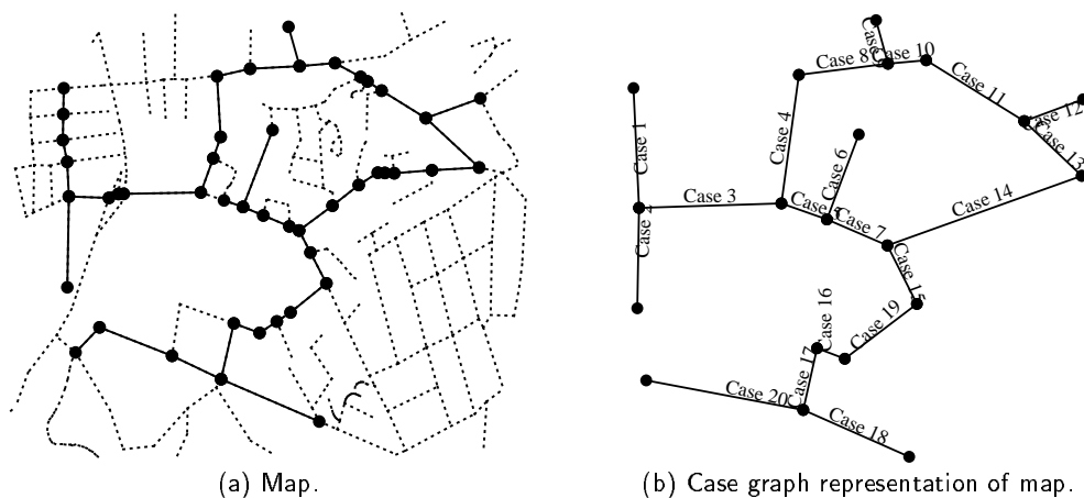
Figure 2: (a) Marked streets and intersections in the map (1% of the complete Pittsburgh map) are locations visited during previous planning. (b) Abstracted cases in the case graph.
