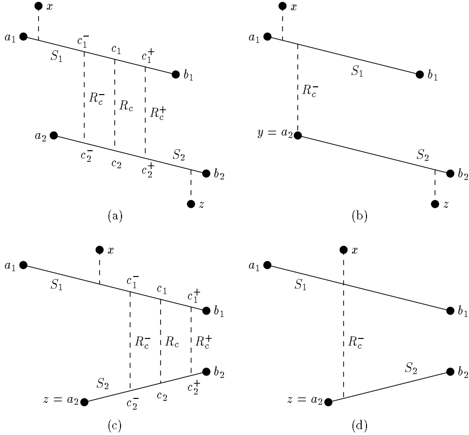
Figure 18: (a) If R is a minimal route from x to z (passing through R_c ), then R^+ and R^- (passing through R_c^+ and R_c^- ) must also be minimal routes from x to z . (b) R^- is a minimal route that passes through an intermediate vertex y . (c) Another example where R , R^+ , and R^- are all minimal routes. (d) R^- is a minimal route that travels one less segment than R .
