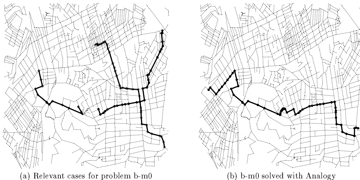
Figure 13: Complex sequential merge, where extra planning is needed around the cases shown in (a) to find the solution shown in (b). (Map shown is 10% of the complete Pittsburgh map.)
