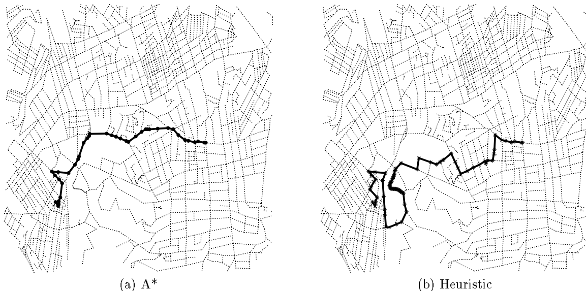
Figure 15: This figure shows how the best-direction-first heuristic can be misled. At left, a solution produced by A*. At right, a solution produced by the best-direction-first heuristic, which always selects the next intersection locally.
