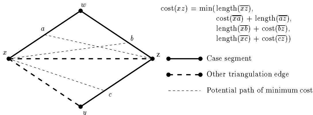
Figure 10: Example of cost calculation for an edge shared by two triangles. Note that the exact positions of a , b , and c depend on the \beta values of the case segments they fall on.
