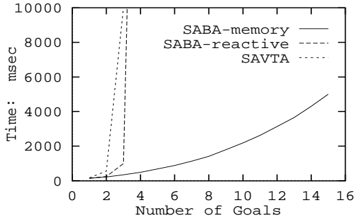
Figure 3: PRODIGY’s performance with different heuristics in domain D^m S^2^*
