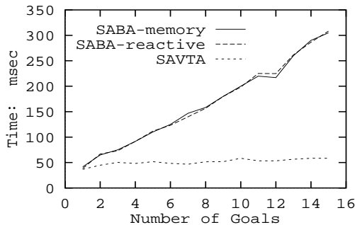
Figure 4: PRODIGY’s performance with different heuristics in domain D^0 -side-effect
