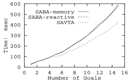
Figure 1: PRODIGY’s performance with different heuristics in domain D^0S^1
