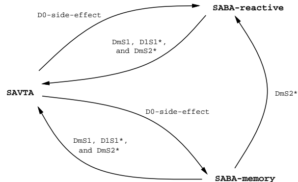
Figure 5: The cyclical dominance relationships of our heuristics. An arrow from x to y means that heuristic x performs better than heuristic y in the indicated domain(s).
