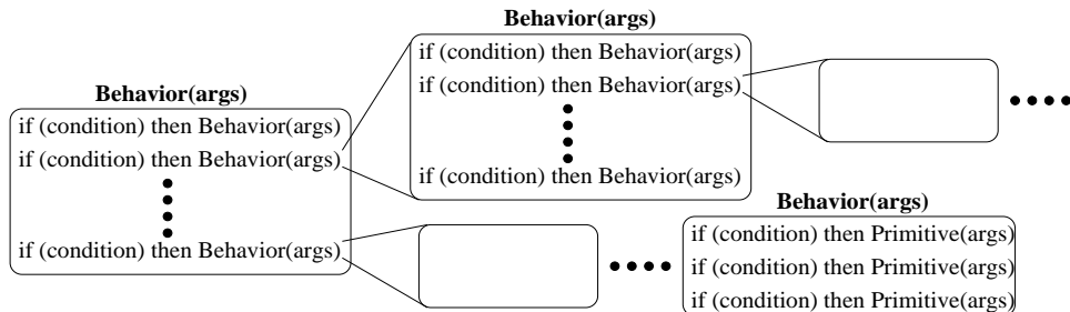
Figure 2: Behaviors in the team member agent architecture. Both internal and external behaviors are organized in a directed acyclic graph.
