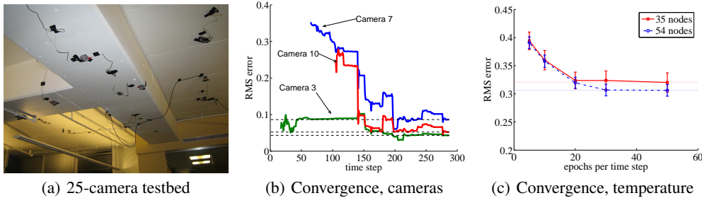
Figure 2: (a) Testbed of 25 cameras used for the SLAT experiments. (b) Convergence results for individual cameras in one experiment. Horizontal lines indicate the corresponding centralized solution at the end of the experiment. (c) Convergence versus amount of communication for a temperature network of 54 real sensors.
