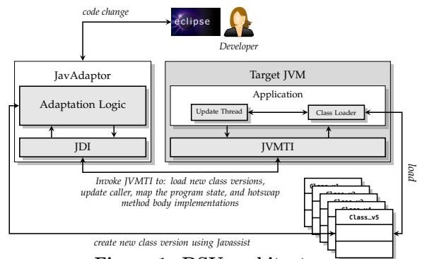
Figure 1: DSU architecture.
