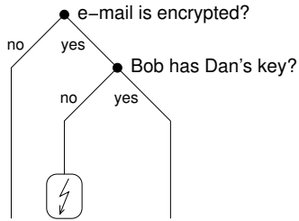
Figure 3: Exploring possible program paths of the e-mail example using a model checker
