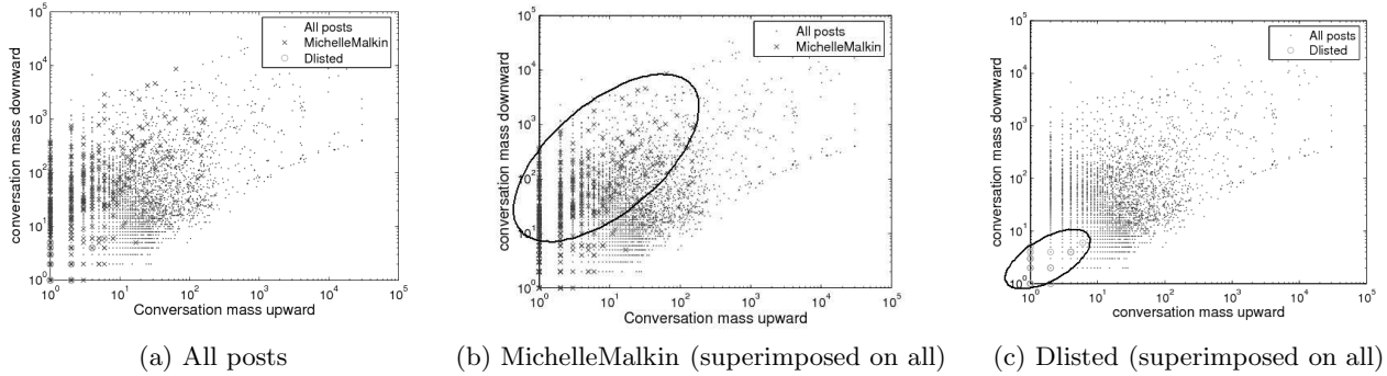
Fig. 4: Conversation mass for posts, an aspect of POSTFEATURES66. The top figure shows the Dlisted and MichelleMalkin clusters superimposed over points for all posts. The next two show the clusters separately, superimposed on all blog points for reference. Ovals are drawn around the main clusters. Note that while there is overlap between posts features of two blogs, they have different centers. This tells us that different blogs maintain different means and variances in conversation masses.
