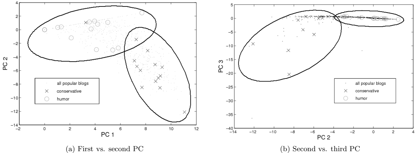
Fig. 3: Principal components for blogs by CASCADETYPE labeled by topic. PC’s were generated by analyzing a matrix of blogs by counts of cascade types. Note that there is a clear separation between conservative blogs (represented by red crosses), and humorous blogs (represented with by circles), both on axes of the first and second PC (a), and on axes of the second and third PC (b). The ovals show the main clusters.
