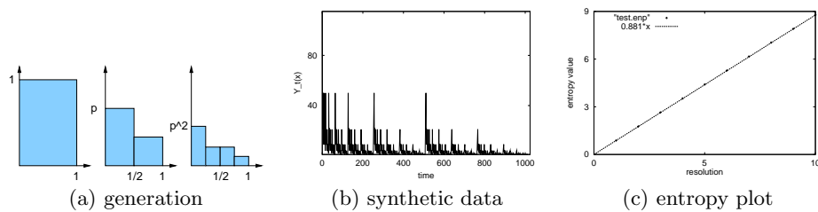
Fig. 6: Illustration of the b -model: (a) the recursive 80-20 procedure in its first three iterations (b) the generated synthetic activity (eg., number of posts, over time) (c) its entropy plot (entropy versus resolution - see text). Because the synthetic input traffic is self-similar, the entropy plot is linear, that is, scale free . Its slope is 0.881, much different than 1.0, which would be the uniform distribution (50-50)
