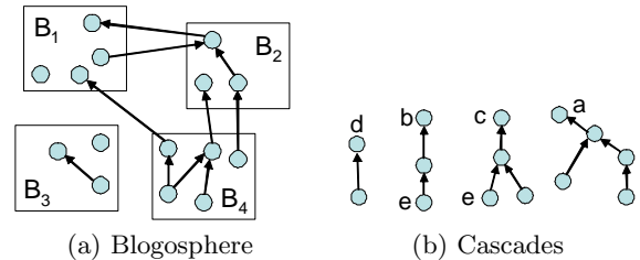
Fig. 1: The model of the blogosphere (a). Squares represent blogs and circles blog-posts. Each post belongs to a blog, and can contain hyper-links to other posts and resources on the web. From the blogosphere, we extract cascades (b). Cascades represent the flow of information through nodes in the network. To extract a cascade we begin with an initiator with no out-links to other posts, then add nodes with edges linking to the initiator, and subsequently nodes that link to any other nodes in the cascade.
