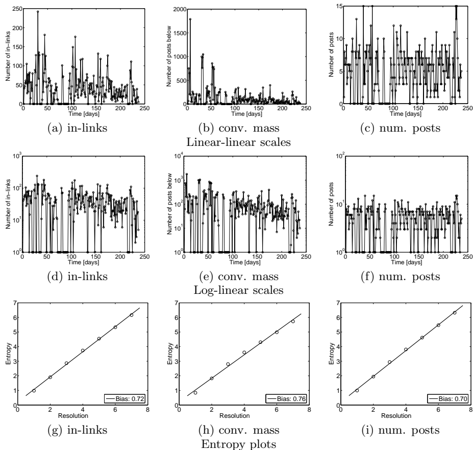
Fig. 5: Time plots are bursty: in-links, conversation mass and number of posts, over time, for the www.MichelleMalkin.com blog. Top row: linear-linear axis; middle row: the 'y' axis is logarithmic. Bottom row shows the entropy plots (see text - entropy versus resolution r' ): they are all linear, which means that the time sequences are self-similar
