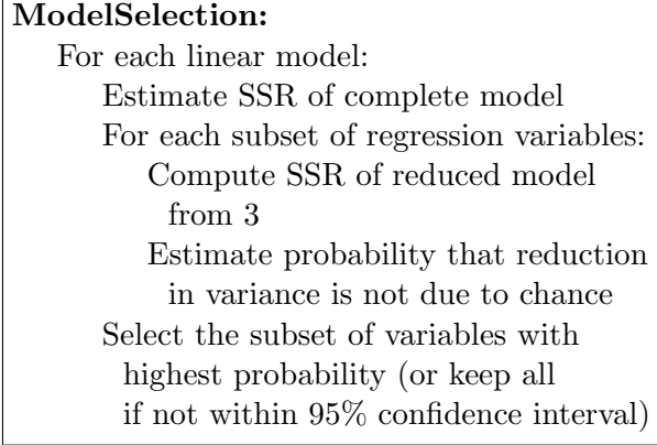
Figure 5: High-level description of basic selection algorithm.
