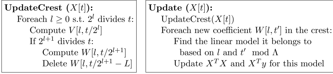
Figure 3: High-level description of update algorithms.
