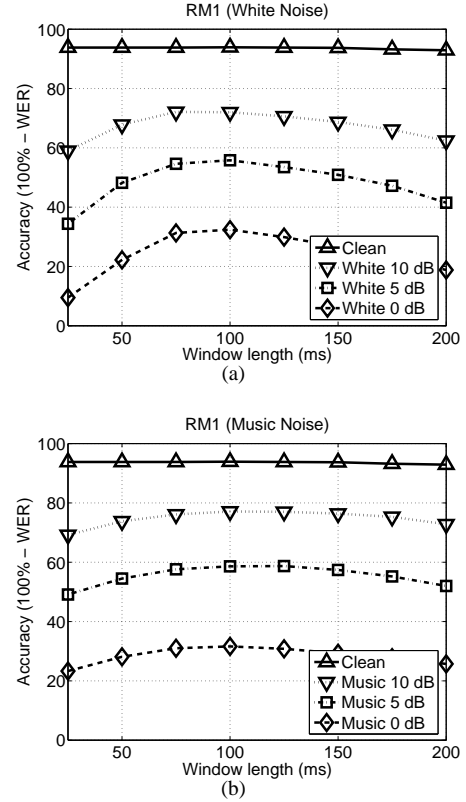
Fig. 4. Speech recognition accuracy as a function of window length for noise compensation corrupted by white noise and background music.
