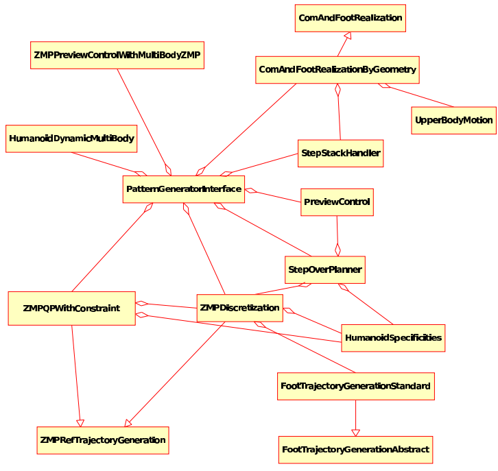
Diagram: class diagram Page 1
