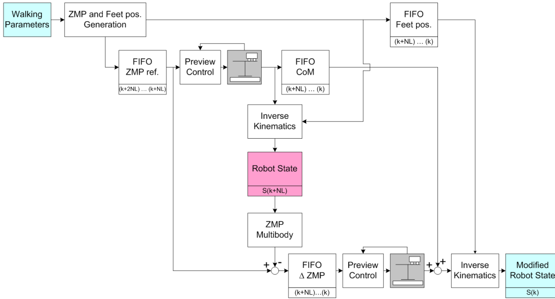
Figure 3: ZMP Preview Control scheme
