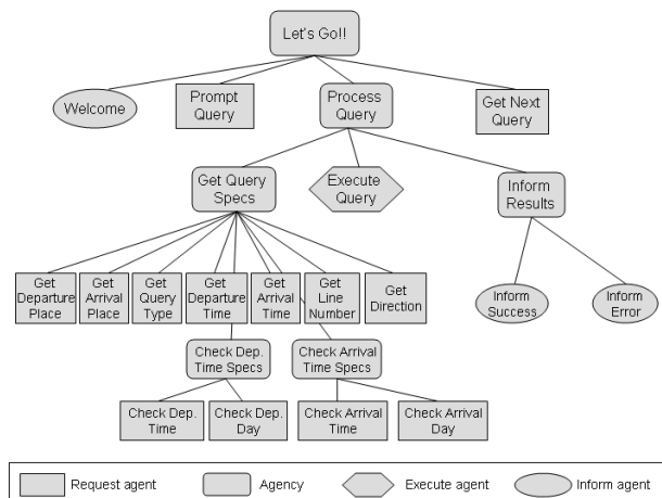
Figure 1: Tree Structure of the Dialog Agents
