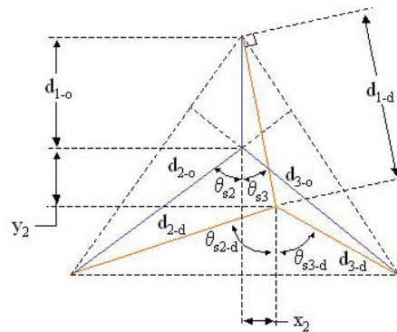
Figure 12. General Spring Displacement Geometry
