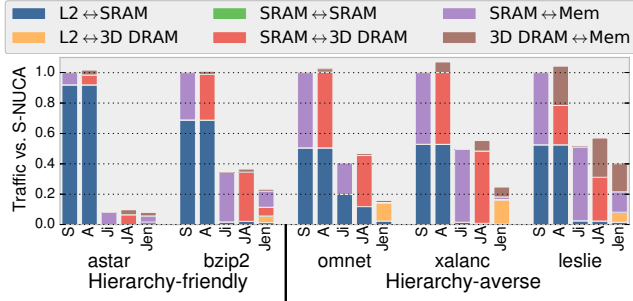
Figure 17: Traffic breakdown on copies of SPEC CPU2006.
