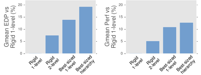
Figure 5: Gmean EDP/perf. of the best rigid hierarchies of 1 or 2 levels vs. application-specific hierarchies of 1 or (up to) 2 levels.
