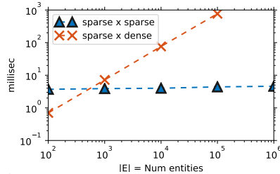
Figure 2: Runtime on a single K80 GPU when using ragged representations for implementing sparse matrix vector product, vs the default sparse matrix times dense vector product available in TensorFlow. |\mathcal{E}| > 10^5 leads to OOM for the latter.
