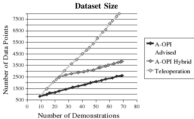
Fig. 8. Dataset size growth with demonstration number.
