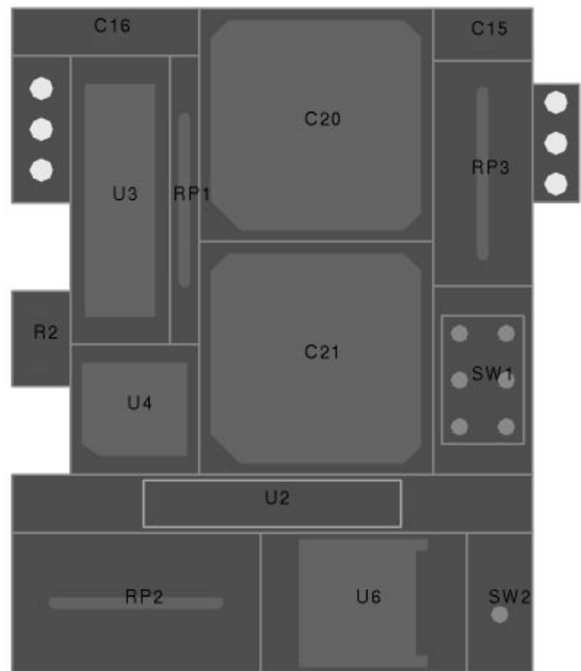
Figure 3: Circuit board layout.
