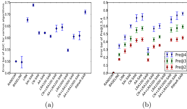
Figure 4: Performance of various algorithms on attribute inference on SEP4. (a) AUC under ROC curves. (b) Pre@2,3,4.
