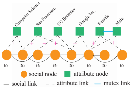
Figure 1: Illustration of a Social-Attribute Network (SAN). The link prediction problem reduces to predicting social links while the attribute inference problem involves predicting attribute links.
