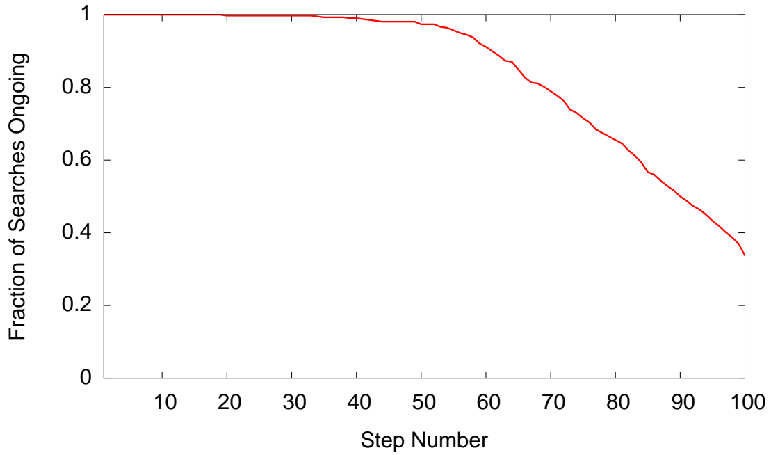
Figure 7: The average fraction of search starts surviving to a given number of steps (i.e., we have not broken out of the intermediate loop begun on line 7 of Algorithm 1) in the Spring 2014 Course Match production run.
