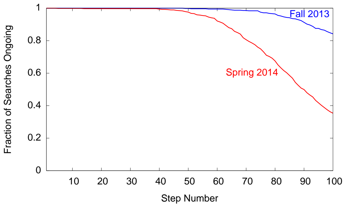
Figure A-7: The average fraction of search starts surviving to a given number of steps (i.e., we have not broken out of the intermediate loop begun on line 7 of Algorithm 1) in the non-production runs using data from the Fall 2013 and Spring 2014 semesters.
