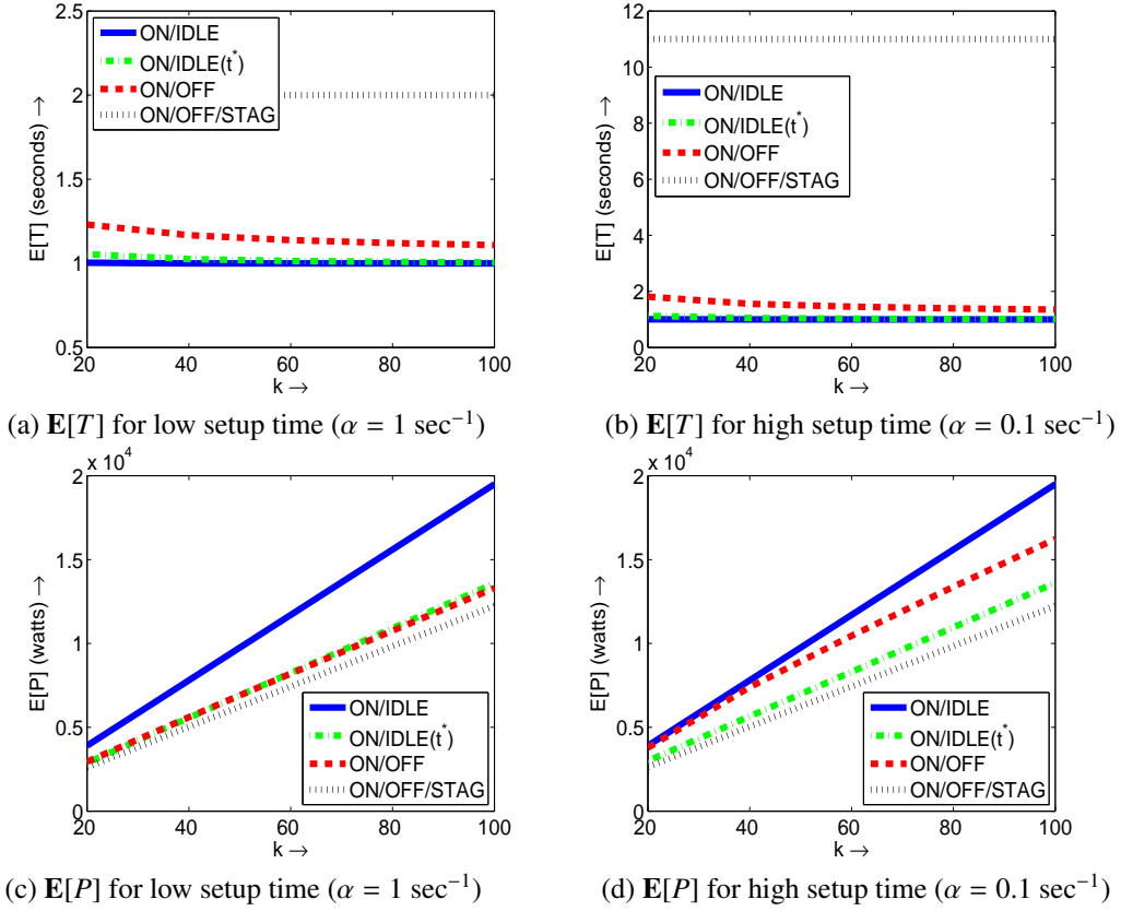
Figure 12: Comparison of E[T] and E[P] for the policies ON/IDLE, ON/OFF, ON/OFF/STAG, and ON/IDLE( t^* ) as a function of k . Throughout, we set \mu = 1 \text{ job/sec} , \frac{c}{k} = 0.5 and P_{on} = 240W .
