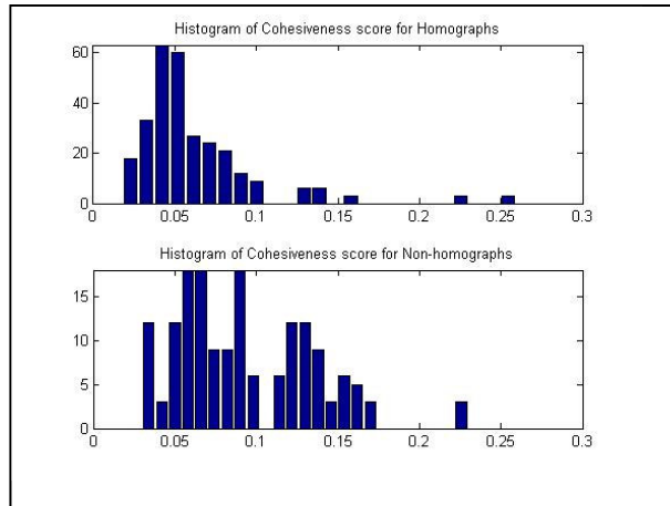
Figure 1. Histogram of Cohesiveness scores for Homographs and Non-homographs.
